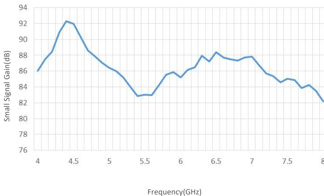
Small Signal Gain vs Frequency
