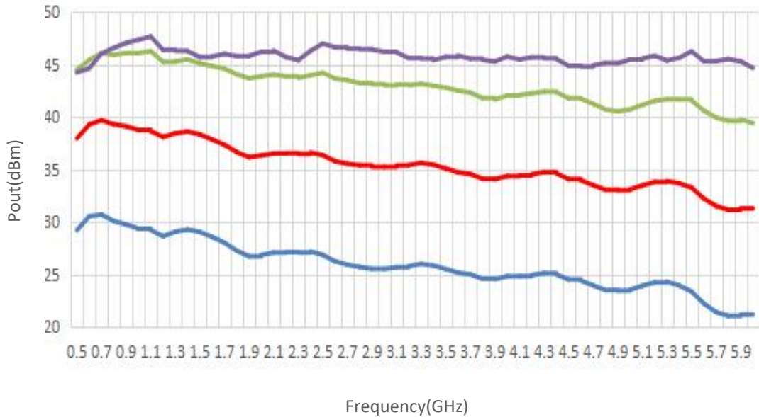
Pout@Equal_Pin
