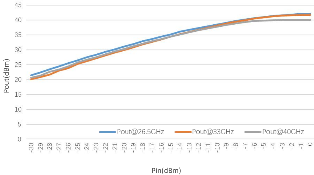
Pout@Equal_Pin
