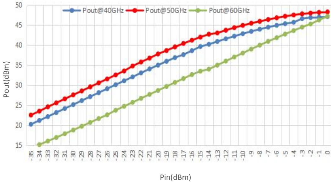
Pout@Equal_Pin
