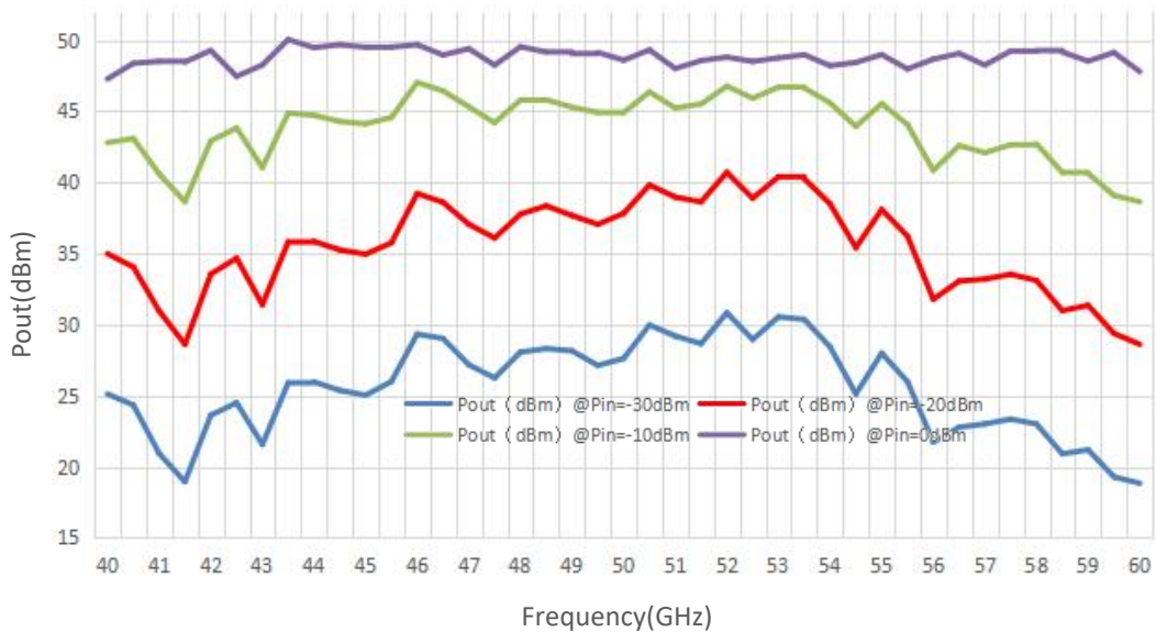
Pout@Equal_Pin
