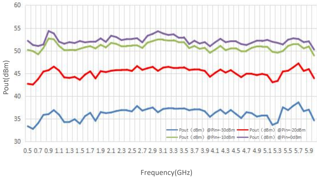
Pout@Equal_Pin
