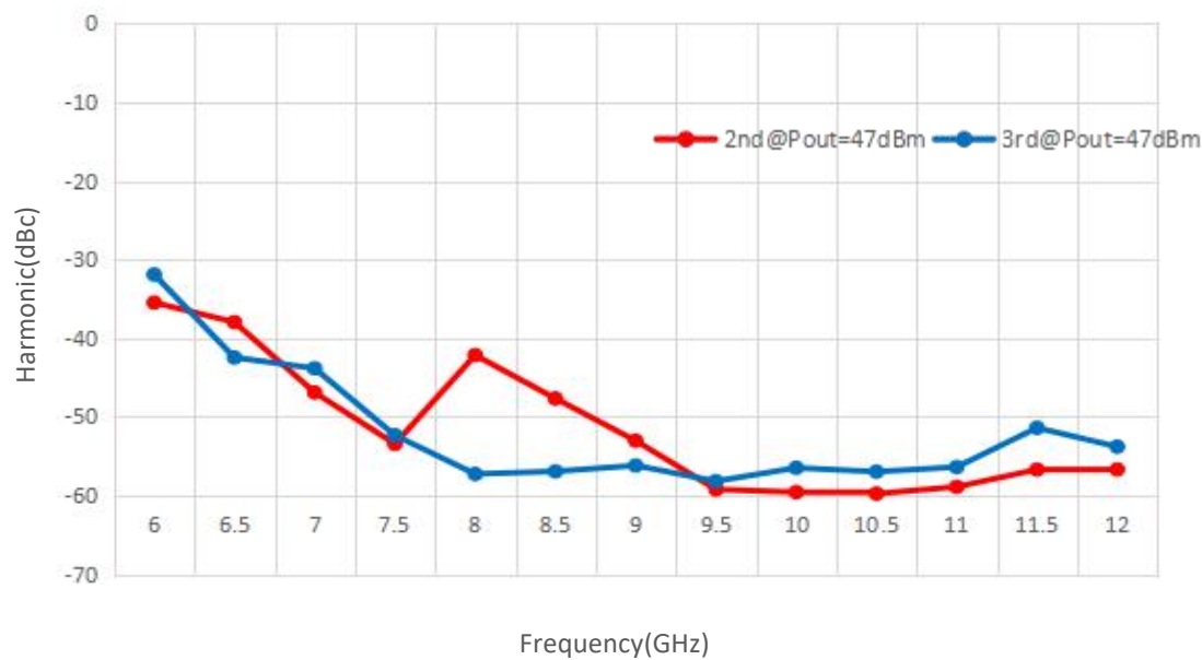
Harmonic vs Frequency
