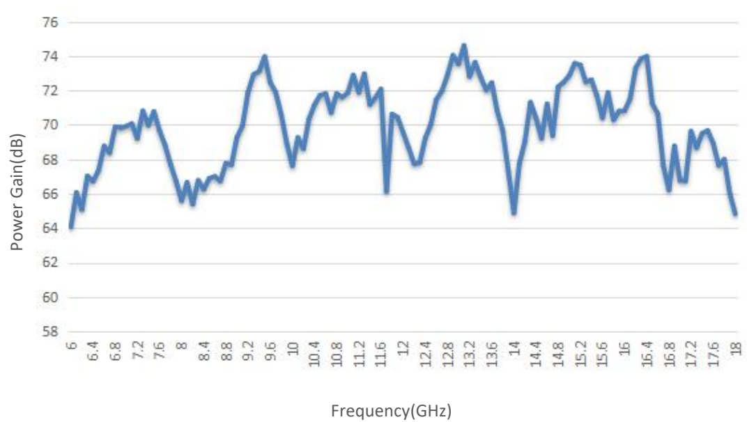
Power Gain vs Frequency
