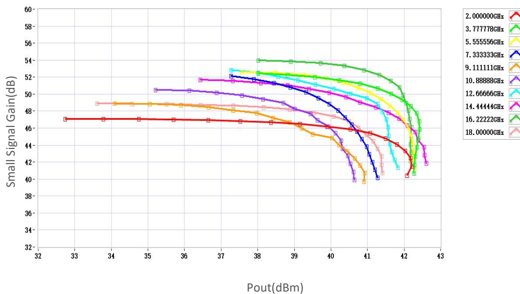
Power Gain vs Output Power
